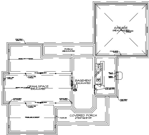
1 FOUNDATION PLAN A-3 SCALE: 1/4"=1'-0"
