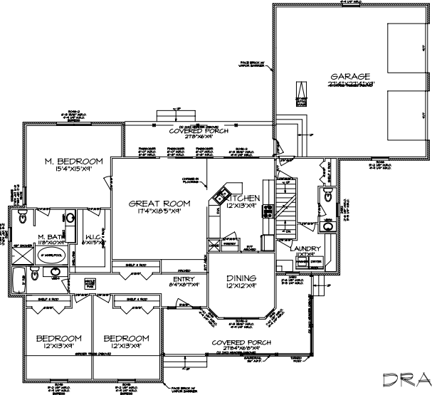
1 FIRST FLOOR PLAN A-1 SCALE: 1/4"=1'-0"
